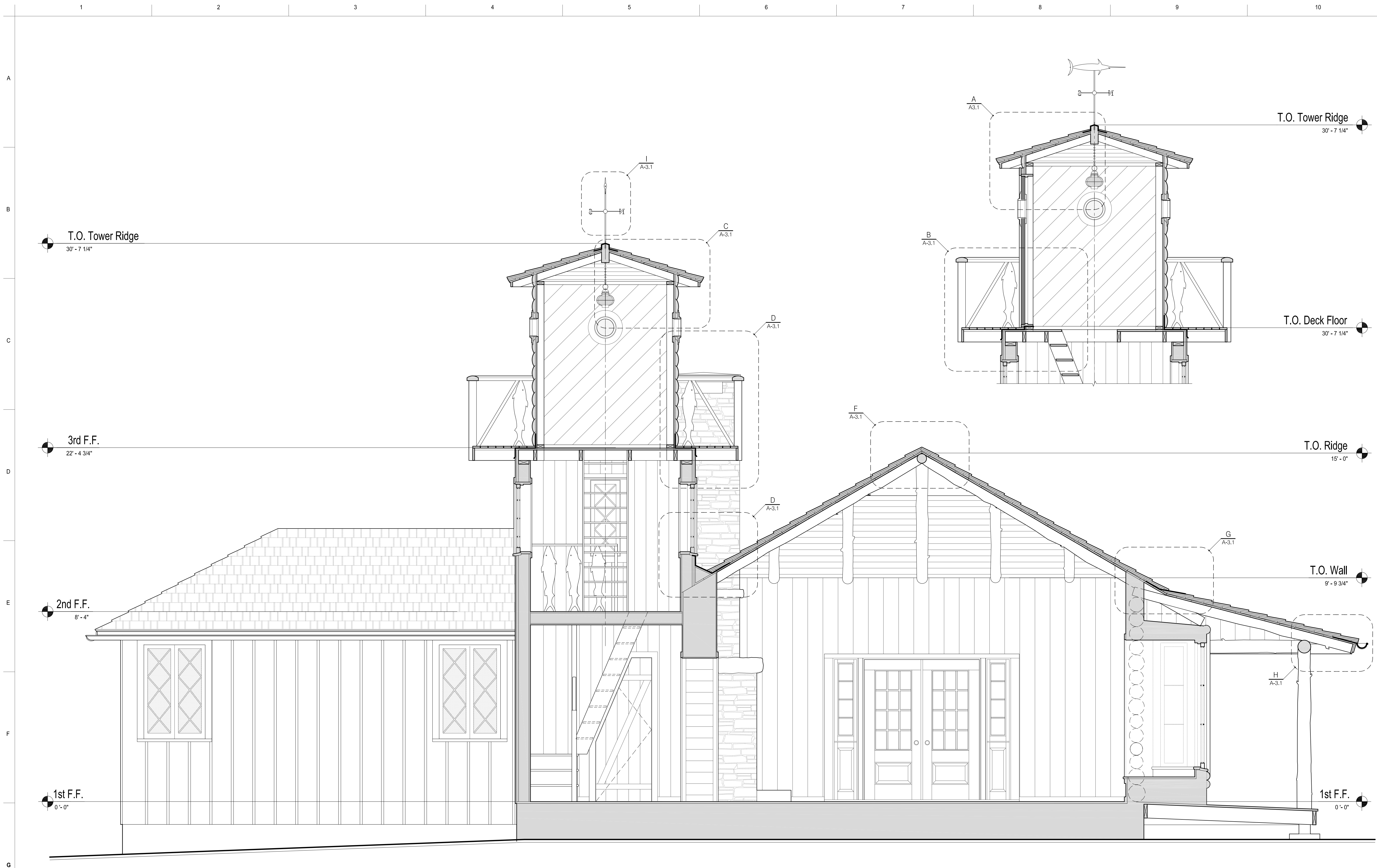
G1 EAST ELEVATION 1/4"=1'-0"
